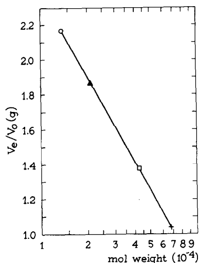
Fig. 1b. Graphical interpretation of the elution data from fig. 1a. \circ RNAase; \blacktriangle CM- \alpha A_1 ; \square ovalbumin; + serum albumin.
