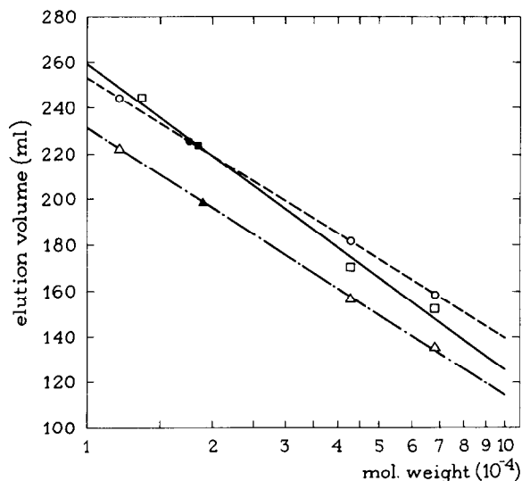
Fig. 2. Graphical interpretation of elution data of separated fractions from a Sephadex G-100 column equilibrated with 6 M urea-0.05 M phosphate buffer at pH 7.6.
